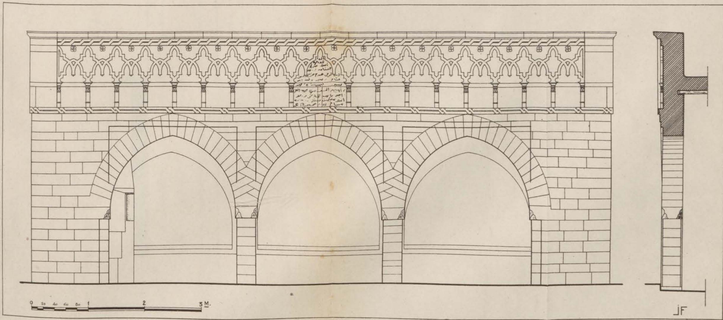
Fig. 74. — Fontaine mérinite, rue Bab Chella. Elevation.
